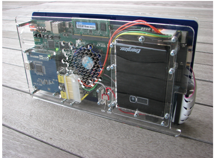
Fig. 2. Tablet construction
